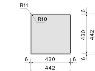
Cut-out size / Flushmount
