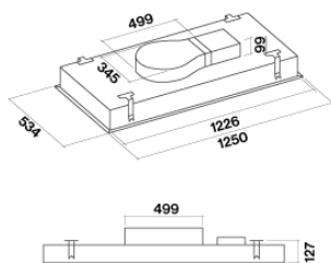
Hood and motor dimensions
