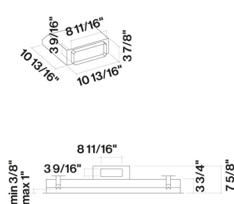
Side view with junction (optional)
