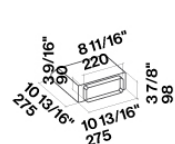
Side view with junction (optional)
