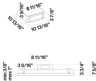
Side view with junction (optional)
