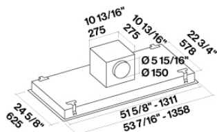
Hood with motor
